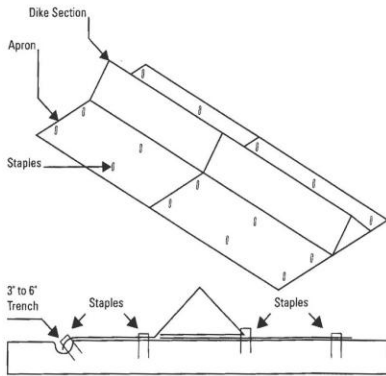
Typical Installation
