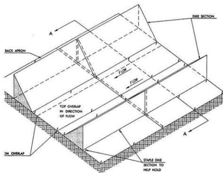
Ditch Liner
